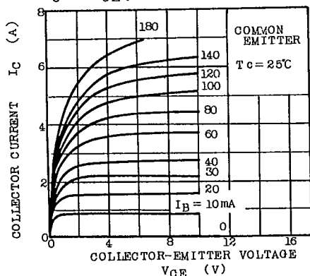
I_C - V_{CE}(\text{LOW VOLTAGE REGION})
